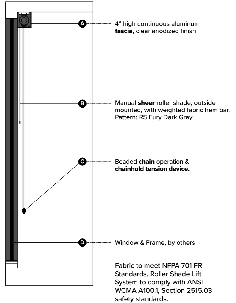
Section
