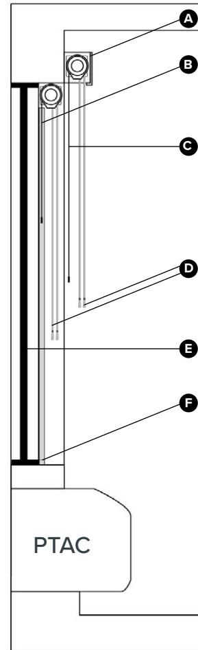
Section
